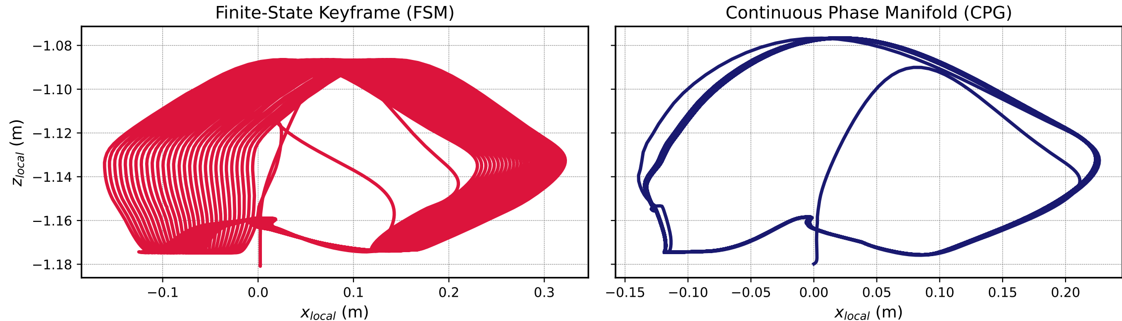
Fig. 1. Cartesian swing-foot phase portraits in the sagittal plane ( x - z ). The discrete Finite-State Keyframe approach (left) yields non-differentiable spatial vertices, whereas the continuous CPG phase manifold (right) generates a C^2 -continuous, smooth limit cycle.
